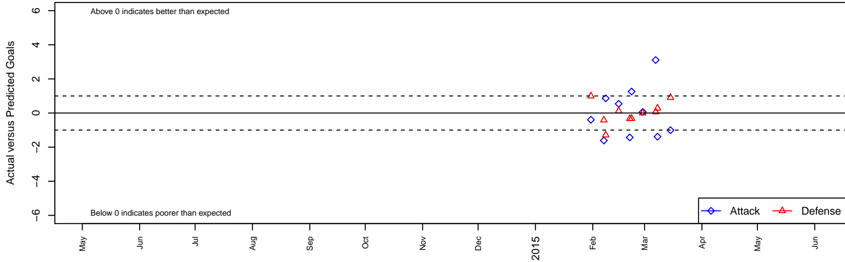
CYSA Timber Barons Green G99 Dots are actual minus expected GF (blue circles) and GA (red triangles). Blue line is smoothed change in attack strength. Red is smoothed change in defense strength.
